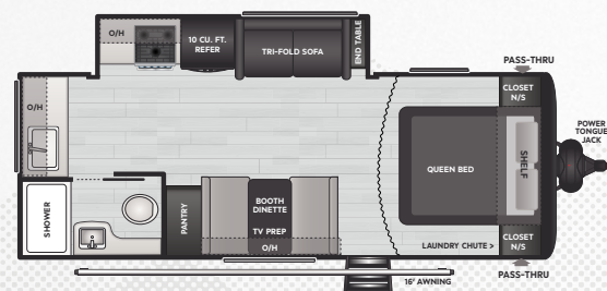
22MLS | WEIGHT 5642 | LENGTH 26' 2"
