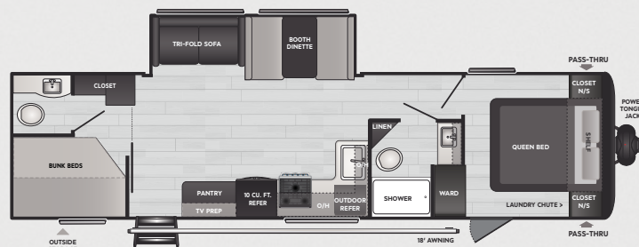
31DBS | WEIGHT 7579 | LENGTH 35' 11"
